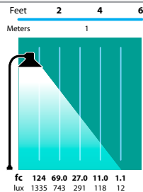
PL-19 Half Spread Photometrics 10 ft. (3.0m) diameter
