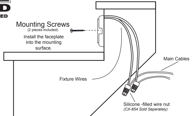
CL-345 Installation Sideview of wall mounting
