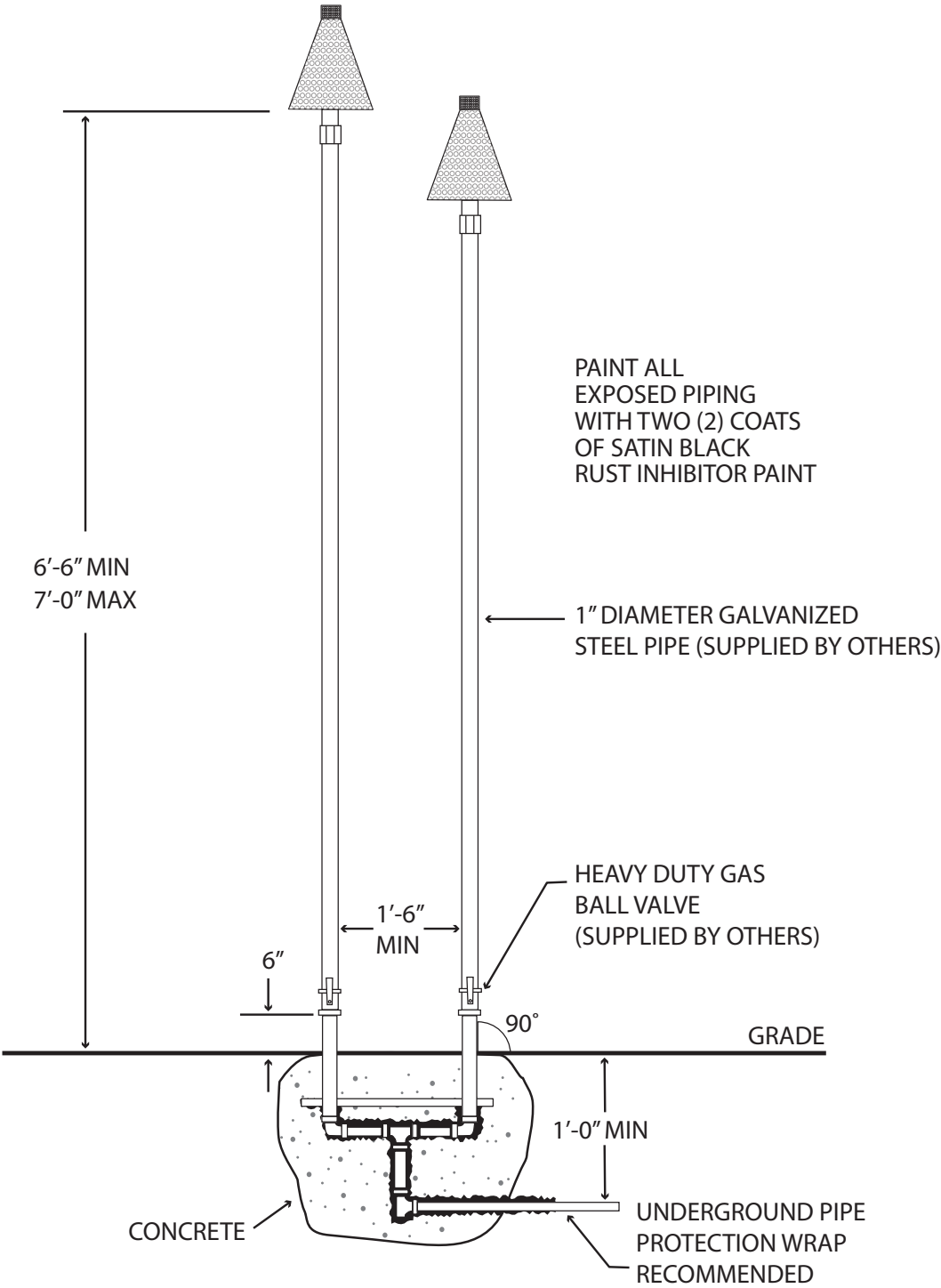
Installation Diagram #1
