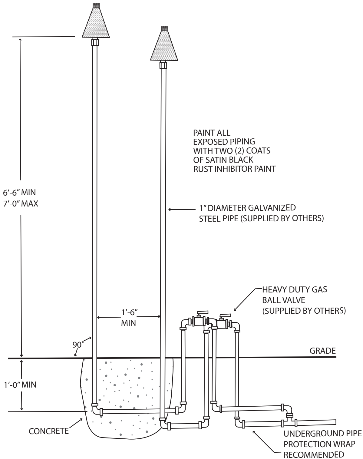
Installation Diagram #2
